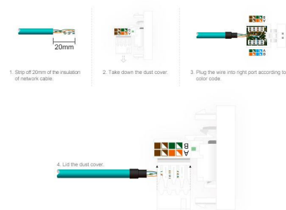
The wiring diagram of COM Socket
